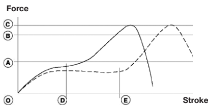
Figure 3 - Force/stroke graph
